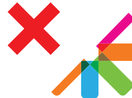
fig. 34: Incorrect consistency
