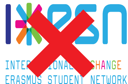
fig. 15: Incorrect scaling
