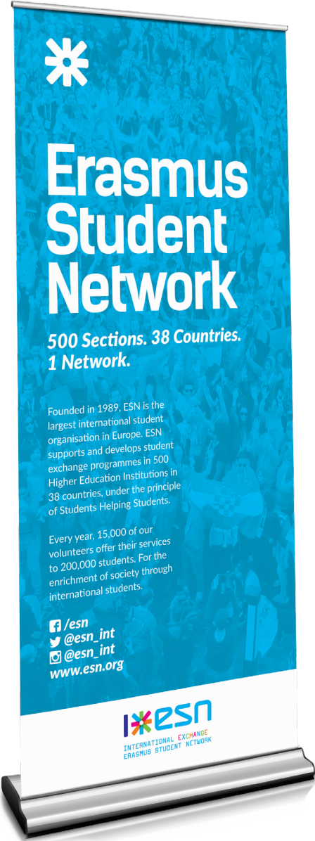
fig. 50: ESN rollup
